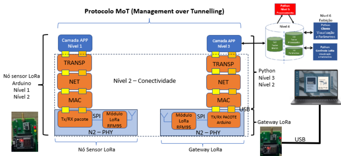
Figura 2 - Framework
